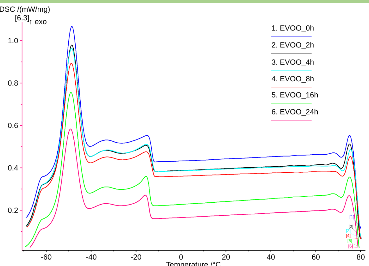
Fig 1. DSC thermogram of EVOO samples heated at 98 °C for 24 hours during cooling from 80 °C to -75 °C at a rate of 10 °C/min.
