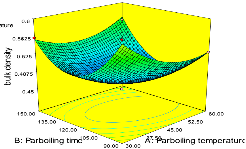
Fig. 1. Response surface plot for bulk density ( \text{g}/\text{cm}^3 ) of breadfruit elubo
