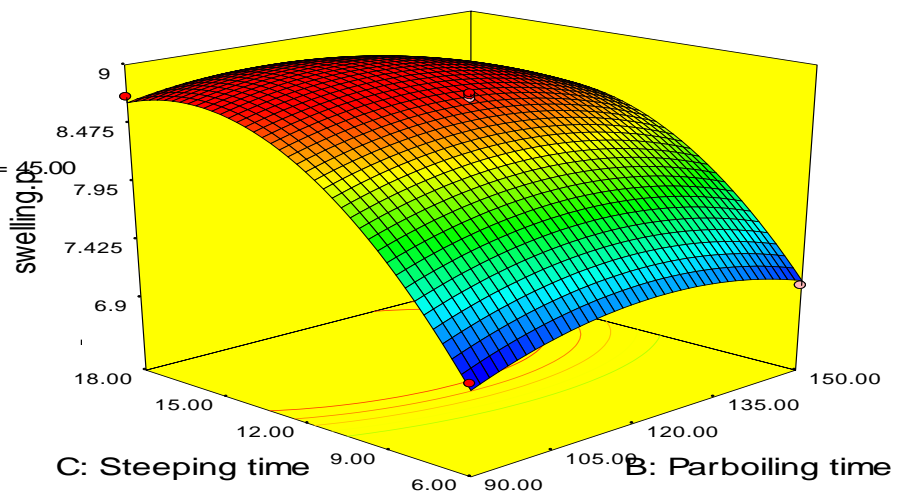
Fig. 3. Response surface plot for swelling power (%) of breadfruit elubo
