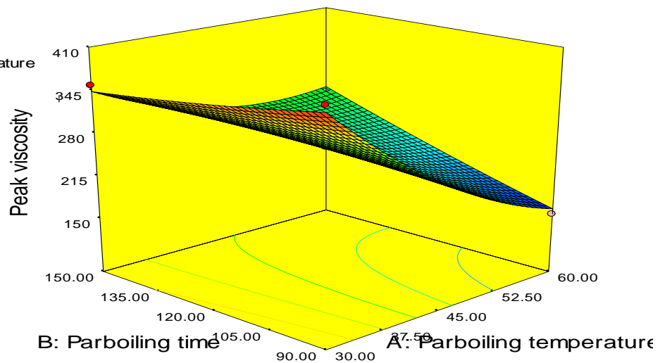
Fig. 6. Response surface plot for the peak viscosity (RVU) parameter of Breadfruit flour at various experimental conditions
