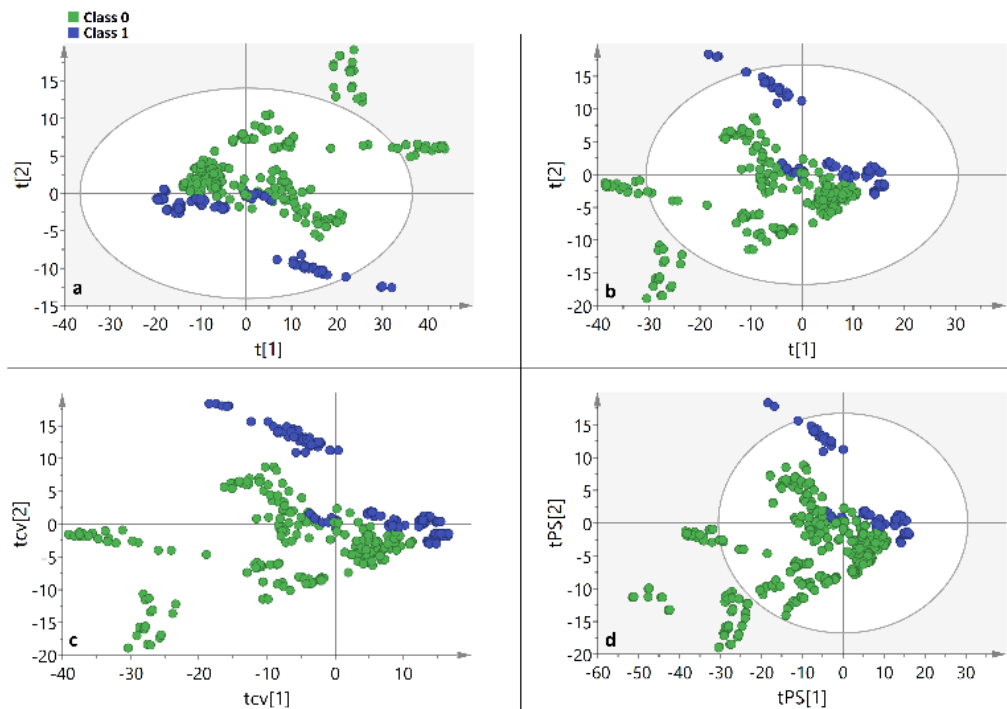
Fig. 4 Class 1 tangerines, Class 0 other samples; a PCA scores scatter plot, b PLS-DA scores scatter plot, c PLS-DA CV scores scatter plot, d PLS-DA predicted scores scatter plot. PCA 3 components, PLS-DA 15 components. t[1] : scores first principal component (PC) or latent variable (LV); t[2] scores second PC or LV; tcv : scores from cross validation; tPS : scores from prediction set
