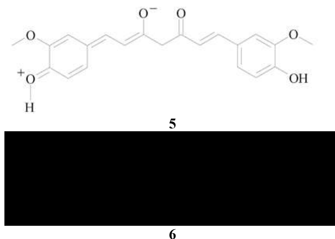
Fig. 3. Zwitterions formed by curcumin
