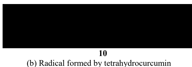
Fig. 4. Radicals formed by curcumin and tetrahydrocurcumin
