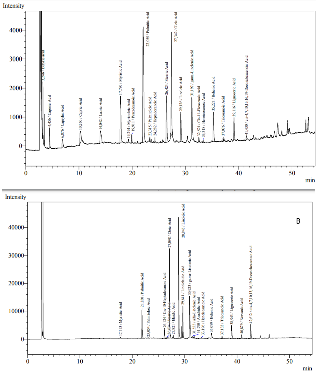
Figure 2. GC-MS chromatograms obtained from plant extracts of A. tinctoria (A) and T. polium (B)
